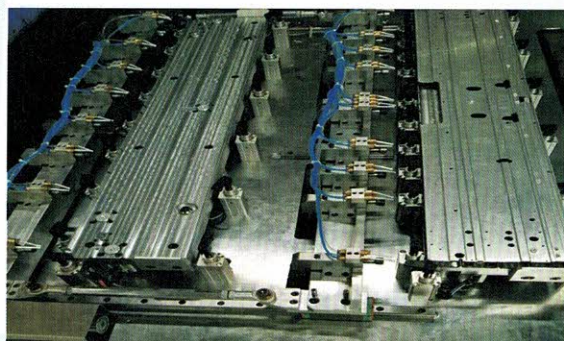
◀ 鋁擠型攻牙系統 aluminum products tapping system
