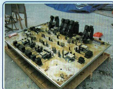
油箱與推油缸 Oil tank & Pusher
